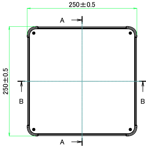
E view
